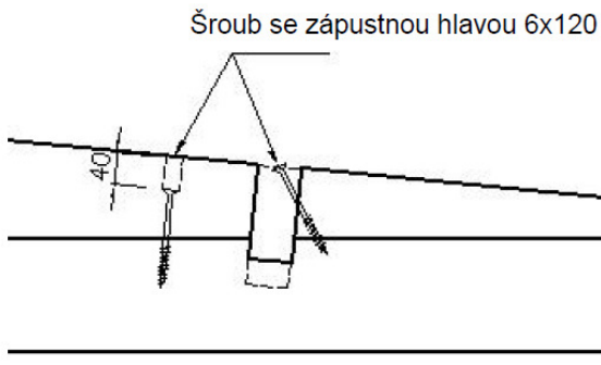
DETAIL C
